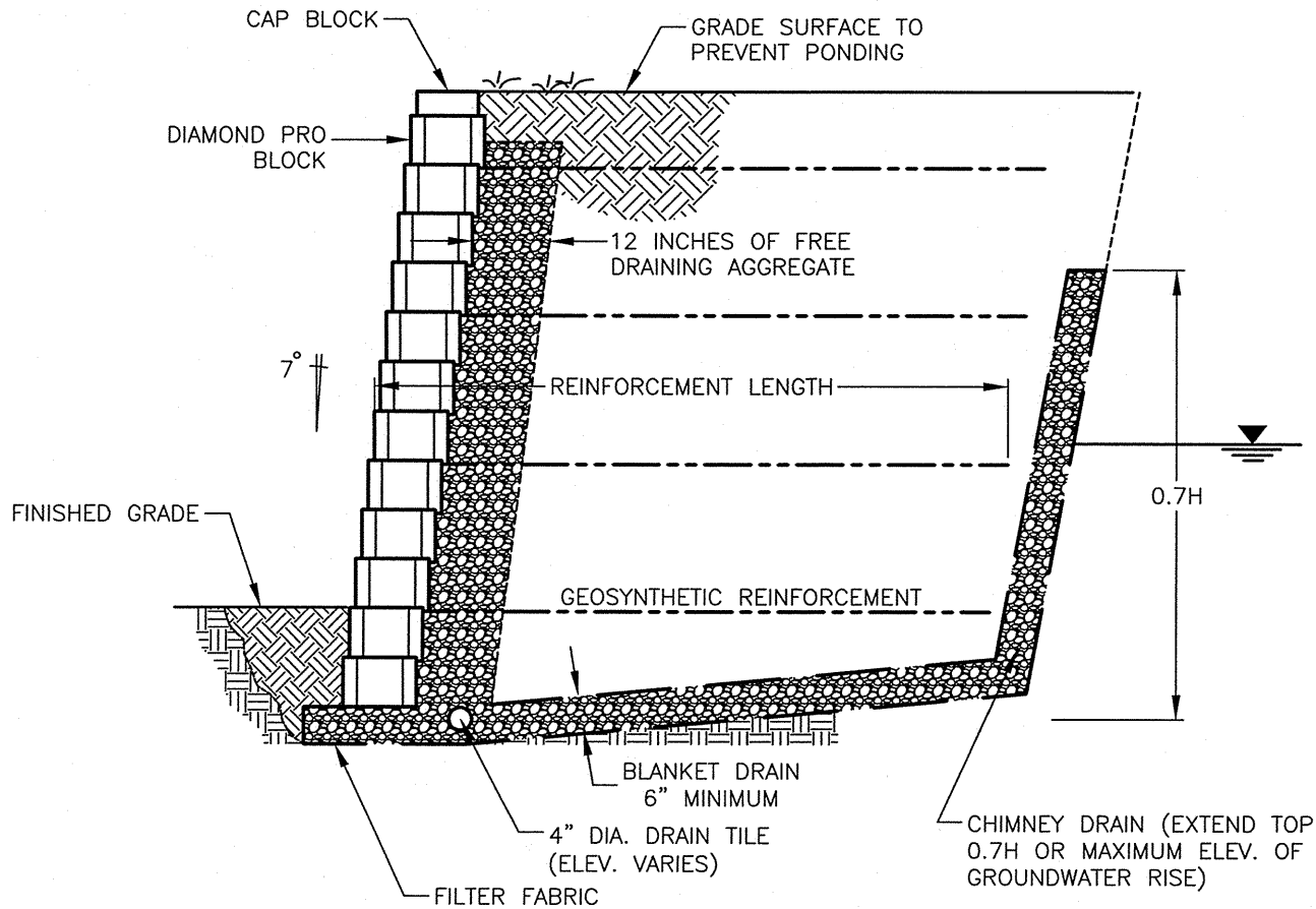
ANCHOR DIAMOND PRO™ X POTENTIAL GROUNDWATER BEHIND WALL WX (SCALE: 3/8" = 1'-0")
