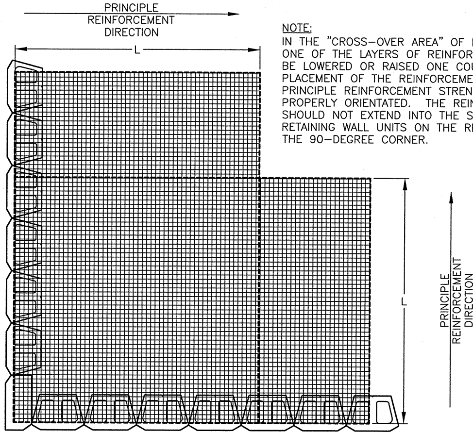
ANCHOR DIAMOND PRO™ X 90-DEGREE OUTSIDE CORNER W/ GRID WX (NOT TO SCALE)
