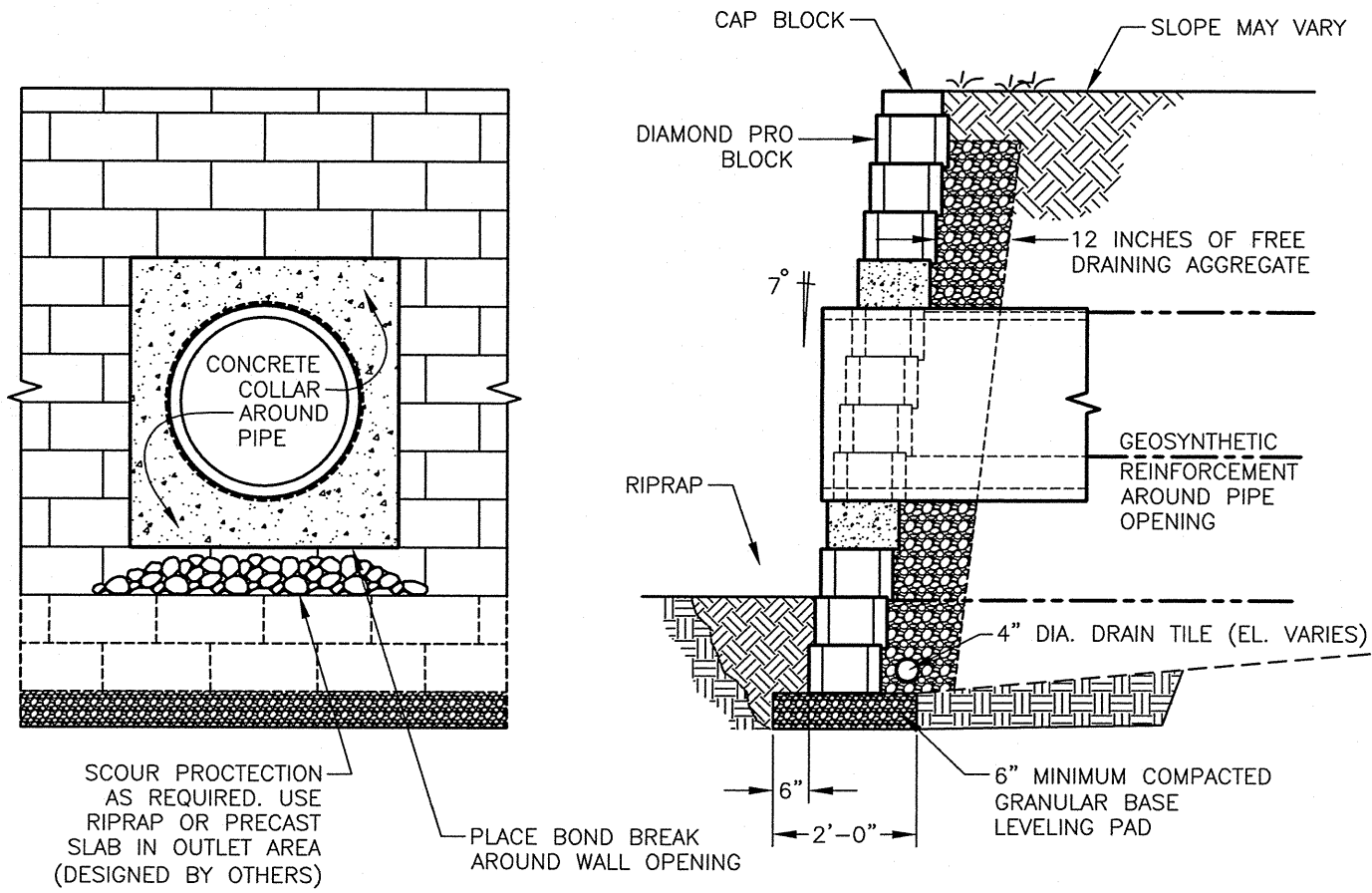
SECTION VIEW
