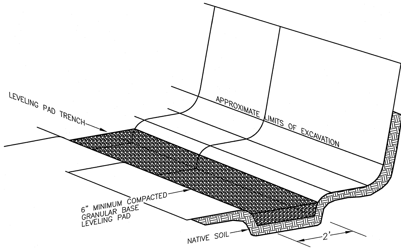
X WX ANCHOR DIAMOND PRO™ TYPICAL BASE PREPARATION (NOT TO SCALE)
